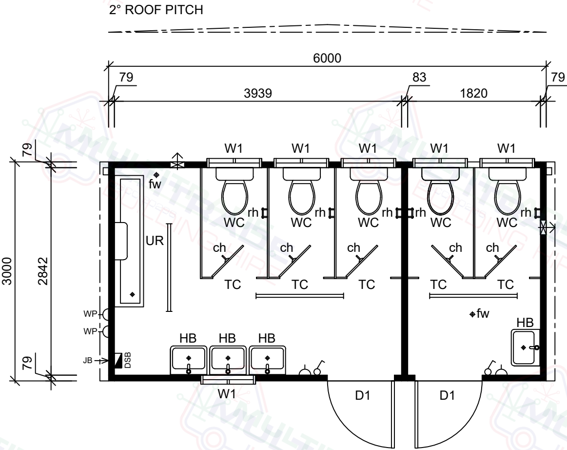
6.0x3.0m Male / Female Toilet - Floor Plan
